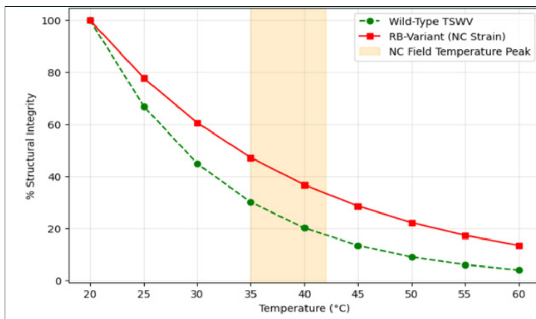
Figure 5: Thermal Denaturation of Viral Envelope Chart: Temperature-dependent stability profile of the TSWV lipid envelope under simulated environmental stress conditions representative of North Carolina field temperatures. The chart compares Wild-Type TSWV, RB (NC Strain), and a modeled NC Field Temperature Peak threshold. Envelope integrity is quantified using a composite stability index derived from lipid order parameters, glycoprotein anchoring retention, and membrane cohesion metrics. RB strains exhibit earlier onset of structural collapse relative to wild-type, with accelerated denaturation observed near peak field-relevant thermal exposure, indicating reduced environmental survivability outside host tissue.
