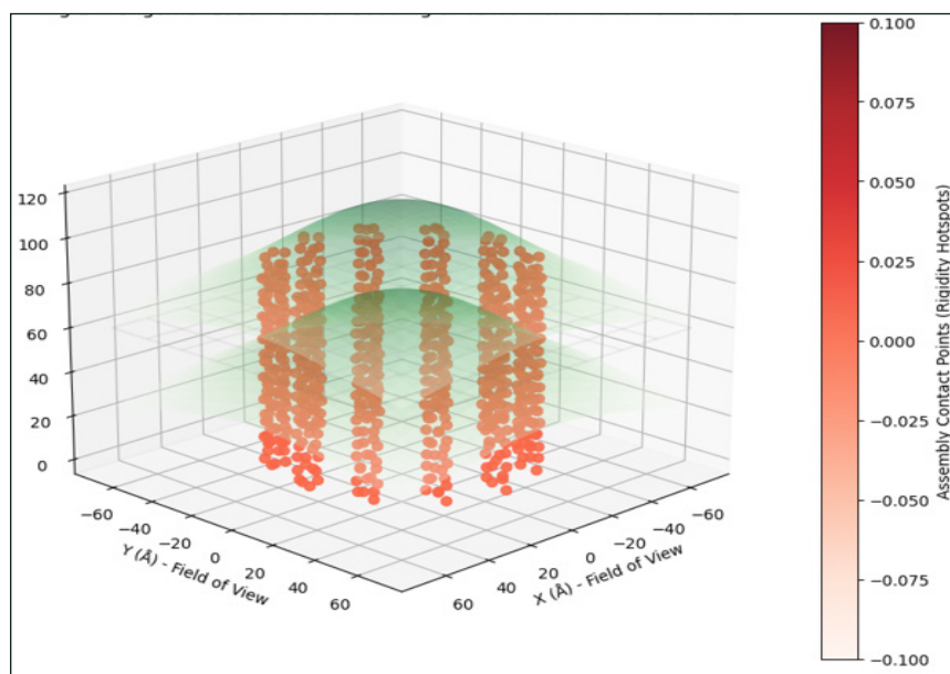
Figure 7: Oligomerization-Driven Budding of TSWV from Plant Membrane (3D Model):
