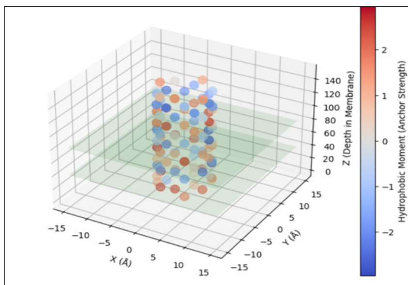
Figure 6: TSWV Glycoprotein TMD in Plant Lipid Bilayer (3D AlphaFold Model): Three-dimensional AlphaFold-derived structural model of the Gn/Gc glycoprotein transmembrane domains embedded within a heterogeneous plant lipid bilayer composed of galactolipids, sterols, and anionic phospholipid clusters. The model visualizes helical insertion depth, membrane curvature effects, and lipid reorganization surrounding protein insertion sites. Hydrophobic transmembrane segments are shown stabilizing within the lipid core, while extracellular domains extend into the solvent-accessible region. Local lipid deformation patterns highlight how glycoprotein anchoring induces nanoscale membrane restructuring critical for viral envelope assembly.
