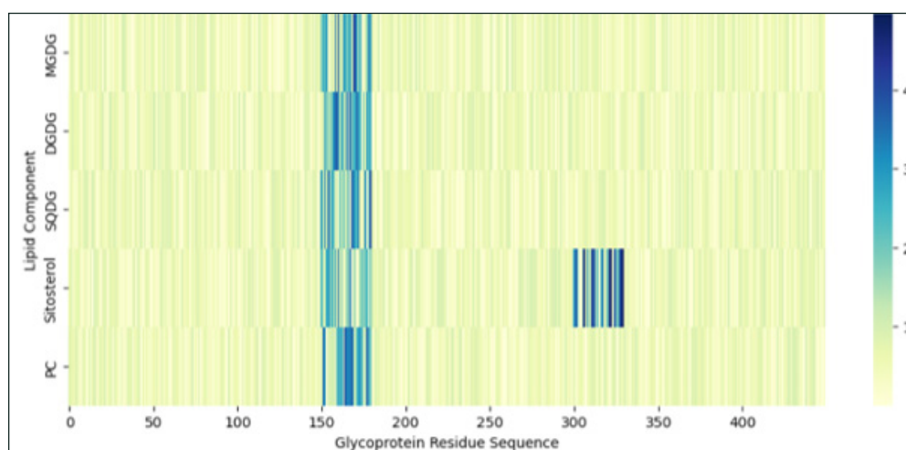
Figure 4: Lipid Density Map (Enrichment of Plant-Specific Lipids): Density distribution map of lipid species incorporated into the TSWV-derived viral envelope following host membrane acquisition. The simulation models preferential incorporation of plant-specific lipids, including galactolipids and sterol-like molecules, into the viral bilayer during budding. High-density regions indicate selective lipid enrichment surrounding glycoprotein insertion sites, suggesting non-random lipid sorting during envelope formation. This spatial enrichment pattern supports the hypothesis that TSWV actively stabilizes its envelope by exploiting specific host lipid microdomains rather than passively acquiring membrane material.
