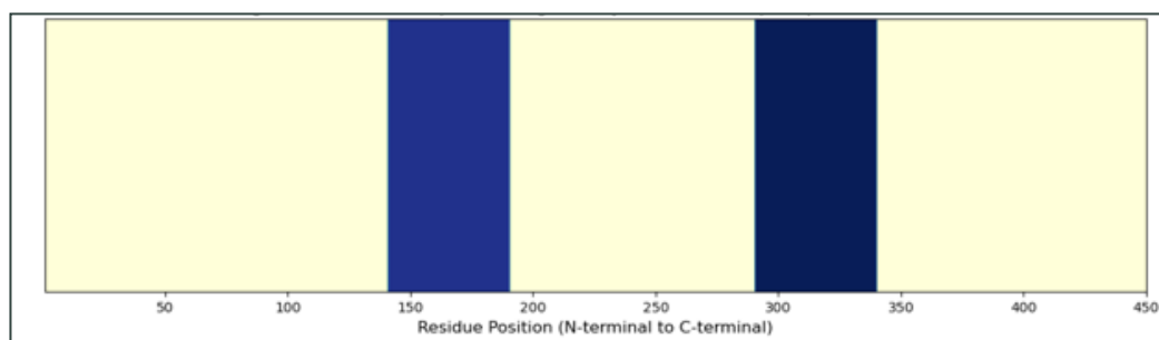
Figure 2: Predicted Lipid-Binding Affinity (Anionic Phospholipid Interaction)
