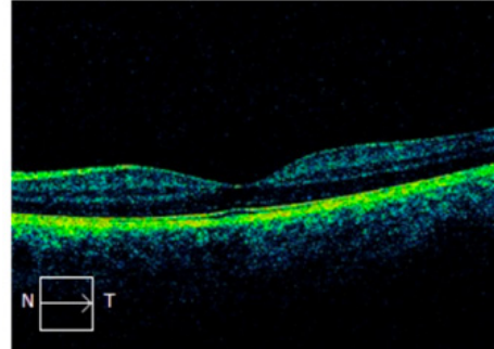
OS Horizontal B-Scan
