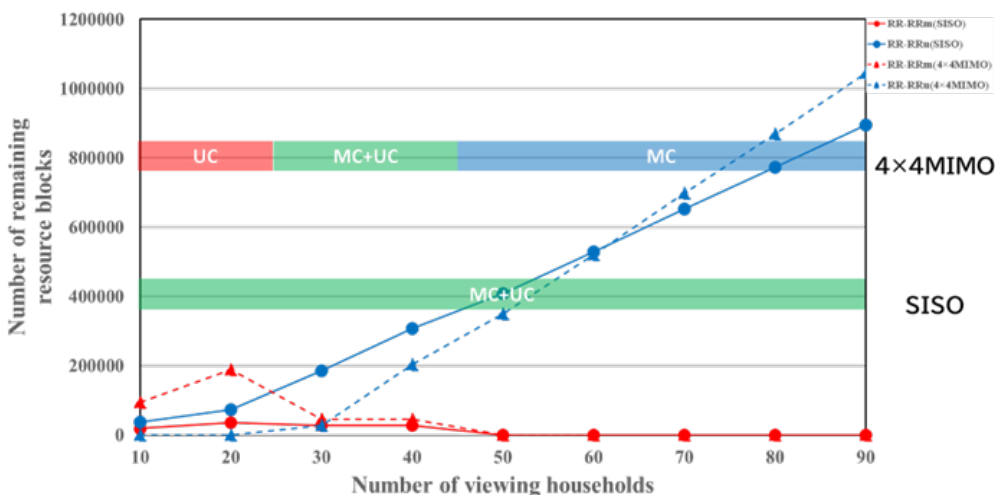
Figure 11: Remaining Resource Block at Radio Interference
