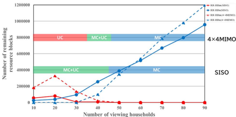
Figure 10: Remaining Resource Block at half-Power Beamwidth of 15°
