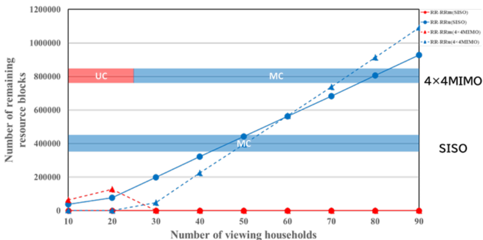
Figure 9: Remaining Resource Block at Half-Power Beamwidth of 30°
